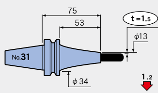
BT30-SLSA10-75 CV
